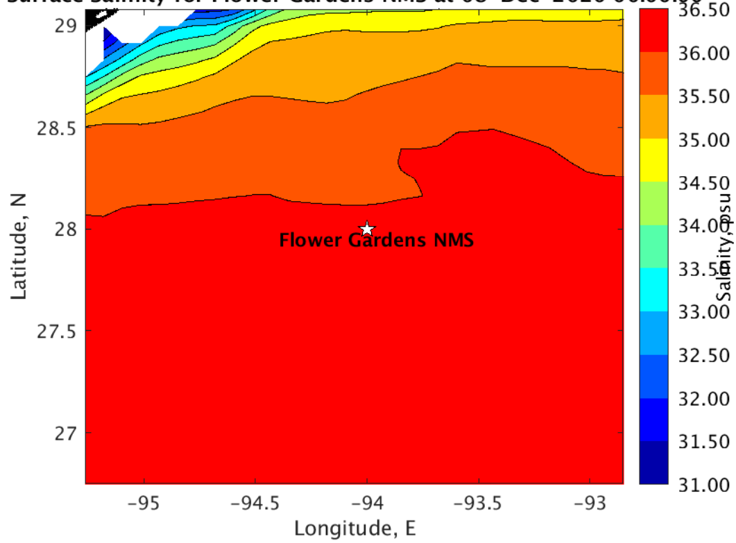
Surface Salinity for Flower Gardens NMS at 08-Dec-2020 00:00:00
